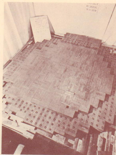
The only photograph of CP-1 known to exist. Taken during addition of 19th layer of graphite. Alternate layers of graphite, containing uranium metal and/or uranium oxide, were separated by layers of solid graphite blocks. Layer 18, almost covered, contained uranium oxide.
