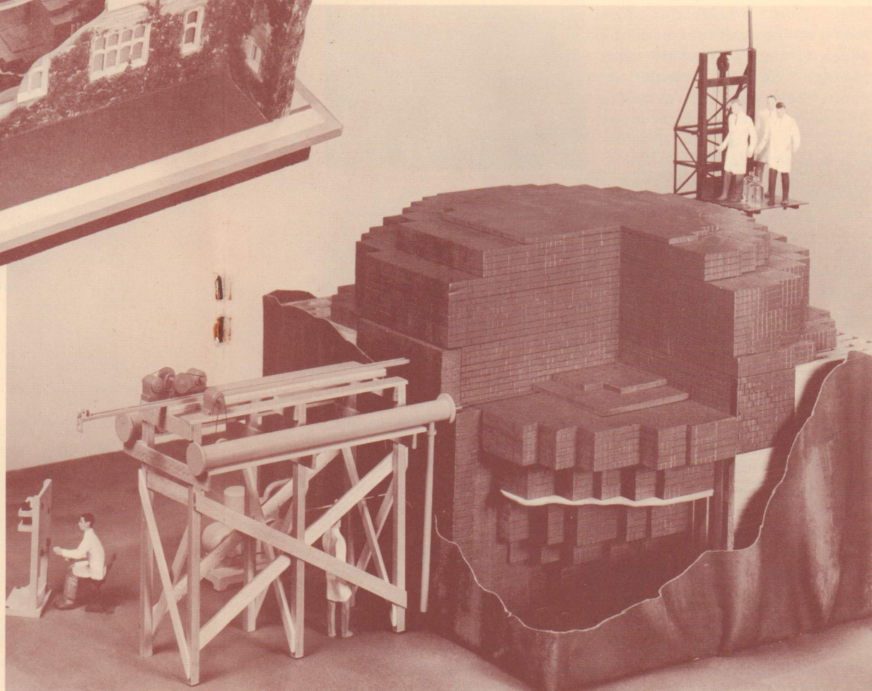
Closeup of scale model of CP-1. A section of the pile is cut away to reveal certain details of construction.
