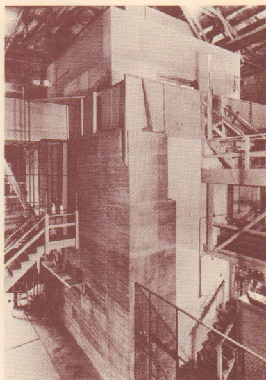
CP-2. The original pile was disassembled early in 1943 and rebuilt with certain refinements and modifications in Argonne Forest Preserve near the present site of Argonne National Laboratory. It was redesignated CP-2 (Chicago Pile Number Two).
