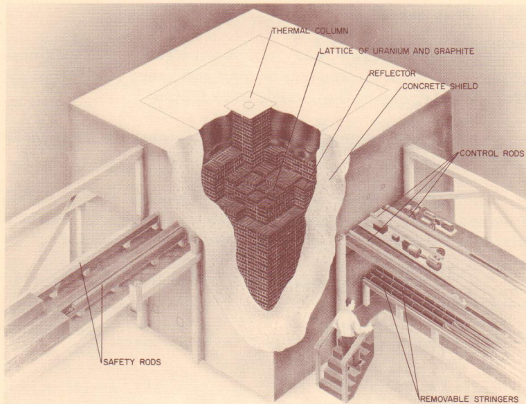
Cutaway view of CP-2
